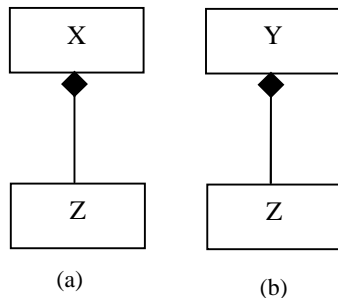
Figure 8. Two diagrams creating an inconsistent Data Model
