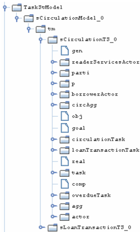
Figure 7. Solution generated by Alloy
