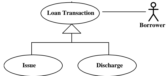
Figure 3. Loan Transaction Task Structure diagram
