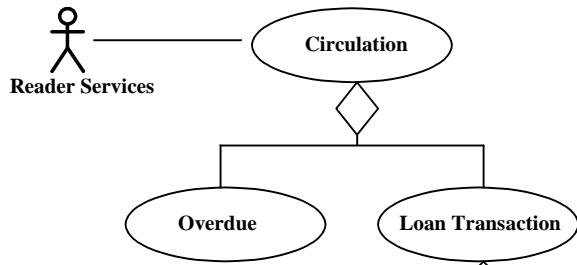
Figure 4. Circulation Task Structure diagram
