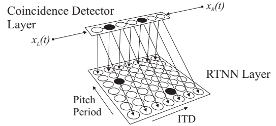
Fig. 2. RTNN (bottom) with coincidence detector layer (top) allowing joint estimation of pitch period and ITD. Each node in the coincidence detector layer is connected to every node in the corresponding RTNN column. Downward connections are only shown for the front and back rows. Recurrent delay loops for the RTNN layer are omitted for clarity. x_L(t) and x_R(t) represent signals from the left and right ears respectively. Solid circles represent activated coincidence detectors.
