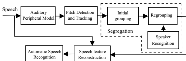
Figure 1 System scheme
