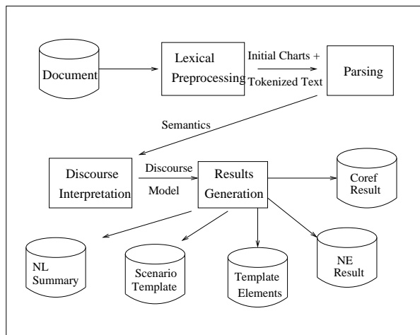
Figure 1: LaSIE System Architecture
