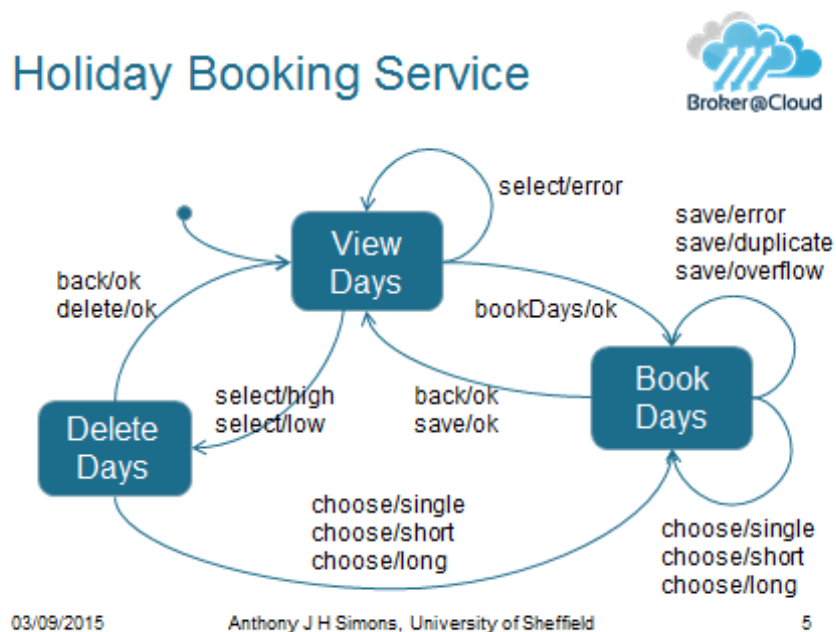
Fig. 1: Visualising the states and transitions of a holiday booking service.
