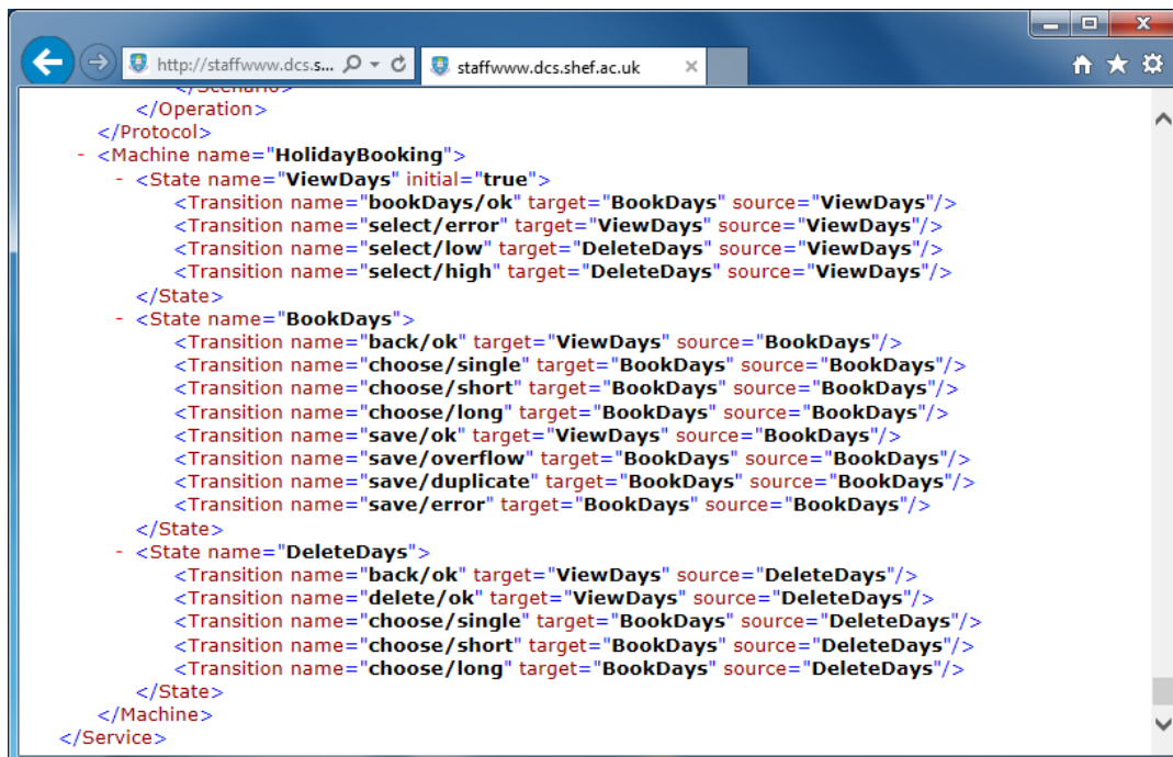
Fig. 7: State machine part of the HolidayBooking specification
