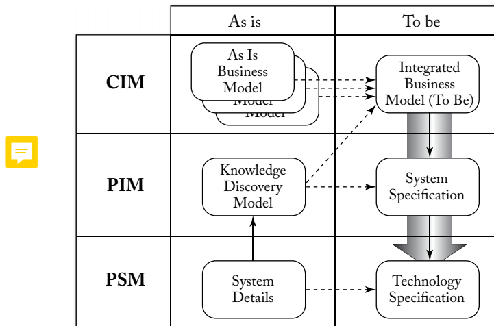
Figure 4.6: Overview of a typical MDRE scenario, as supported by ADM tools.
