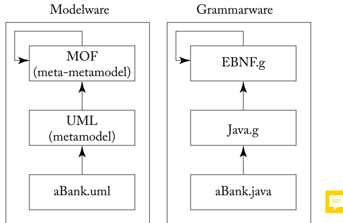
Figure 2.6: Modelware vs. Grammarware.
