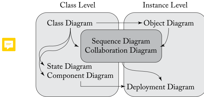
Figure 6.3: Dichotomy between class- and instance-based models in UML.
