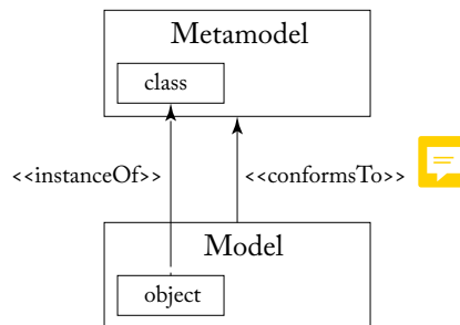
Figure 2.4: conformsTo and instanceOf relationships.
