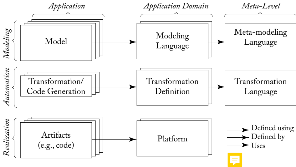
Figure 2.2: Overview of the MDSE methodology (top-down process).
