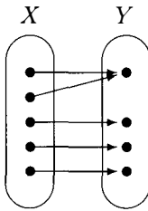
surjective but not injective
