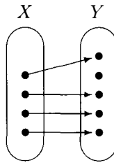
injective but not surjective
