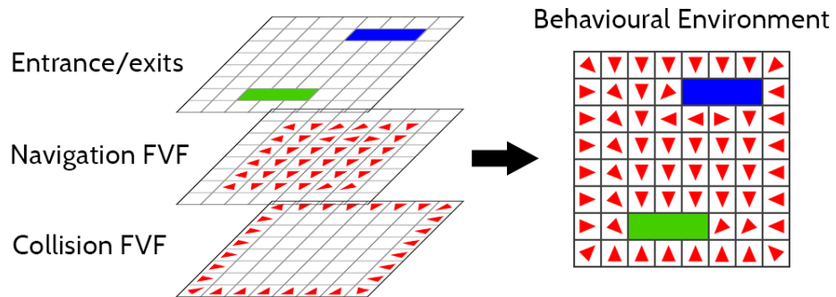
Figure 3: Layered FVFs within the pedestrian simulation program.
